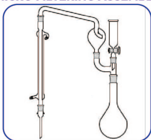
KJELDAHL DISTILLATION
