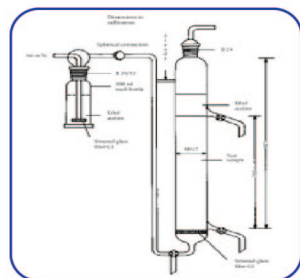
GAS STRIPPING APPARATUS
