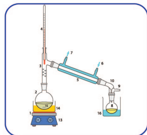
DISTILLATION
