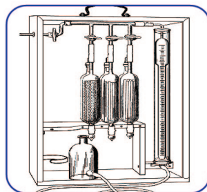
ORSAT GAS ANALYSIS
