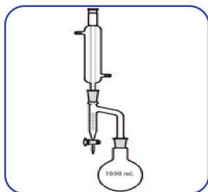
DEAN AND STARK APPARATUS
